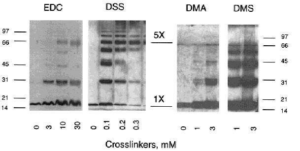
Fig. 3. Crosslinking of purified MscL-6His in OG. The tag-purified MscL protein was transferred into buffers compatible with each crosslinking agent. The agents used were 1-Ethyl-3-(Dimethylaminopropyl) carbodiimide (EDC), disuccinimidyl suberate (DSS), Dimethyl suberimidate (DMS) and Dimethyl adipimidate (DMA) for 1 hr. Crosslinked products were separated by SDS-PAGE and visualized with either Coomassie Blue (left panels) or silver staining (right panels).
